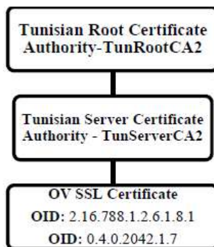
Figure 1- TunRootCA2 hierarchy
